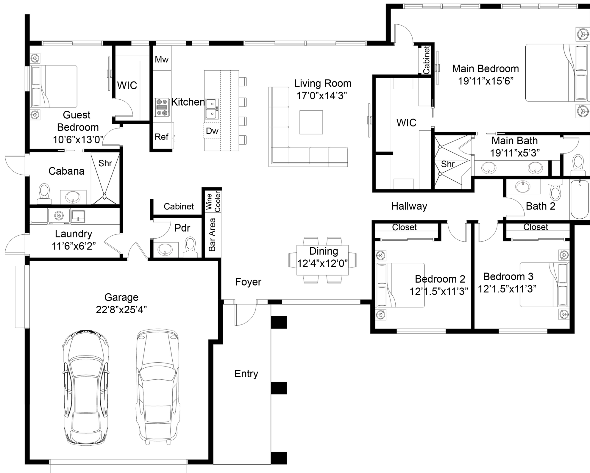
FLOOR PLAN
